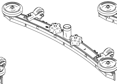
30 INCH SQUEEGEE ASSEMBLY 150-7180
